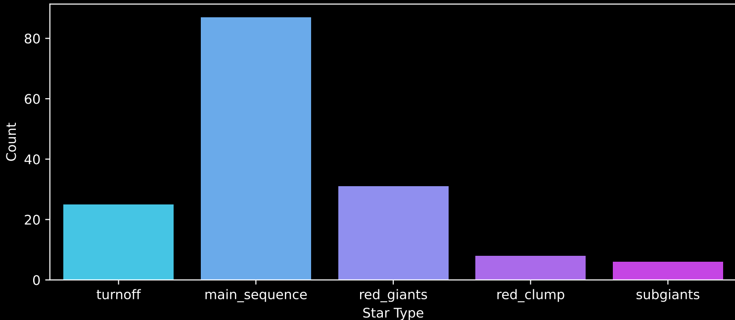
APOGEE DR17 Field: [046+38_MGA] Count plot of Star Type
