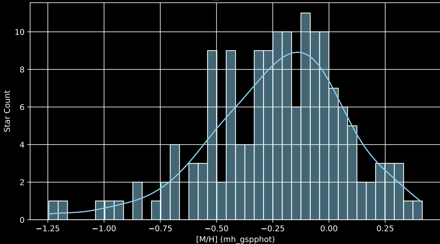
APOGEE DR17 Field: [046+38_MGA [M/H] (mh_gspphot) (n= 156)
