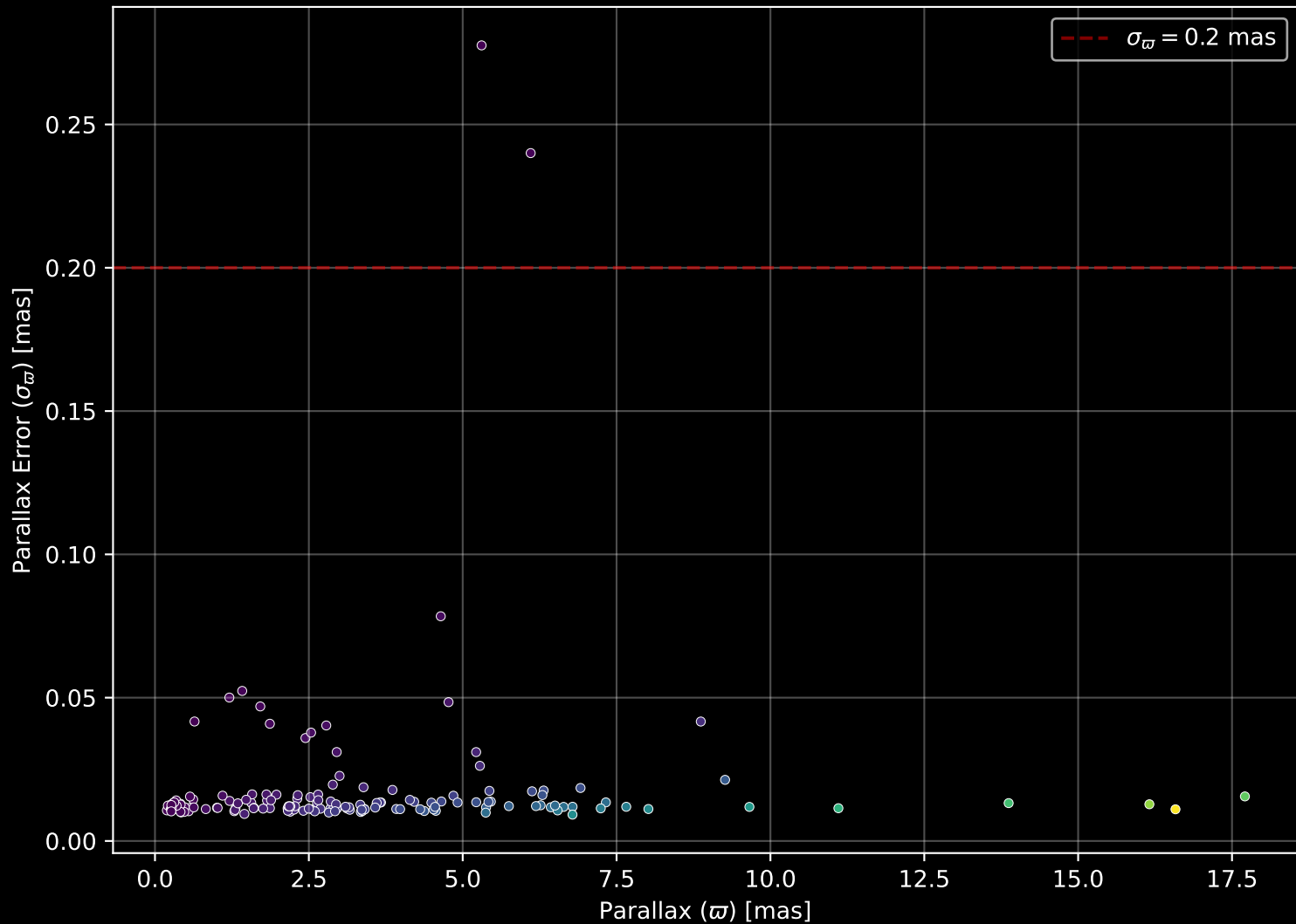
APOGEE DR17 Field: [046+38_MGA] Parallax Quality (n= 157)
