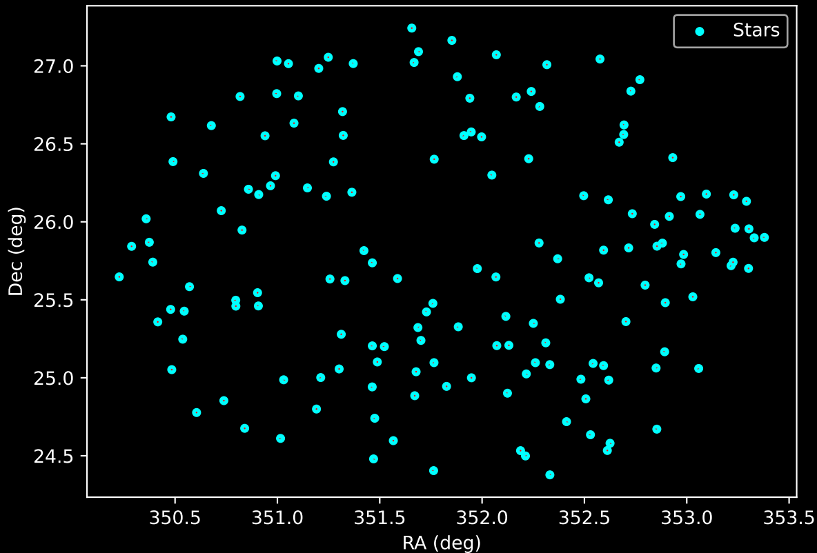
APOGEE DR17 Field: [046+38_MGA] Proper Motion Vectors for Gaia Star Field (n= 157)
