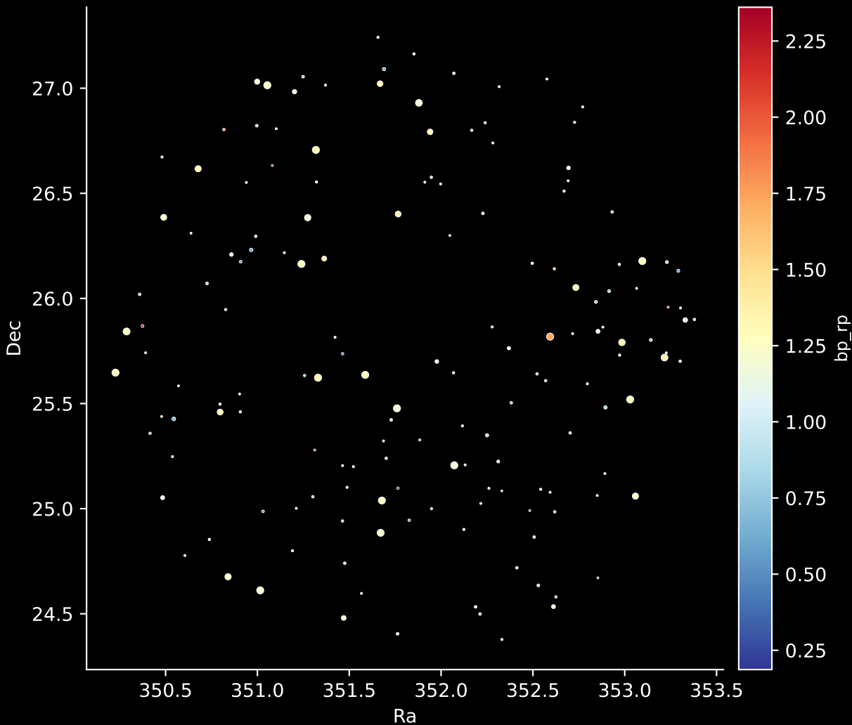
APOGEE DR17 Field: [046+38_MGA] Stars: 157
