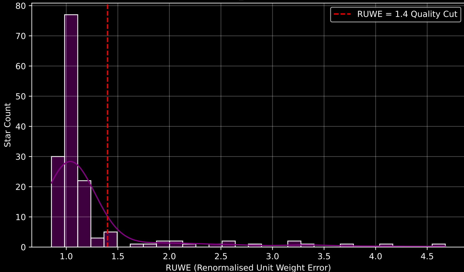
GAPOGEE DR17 Field [046+38_MGA] RUWE Distribution (n= 154)
