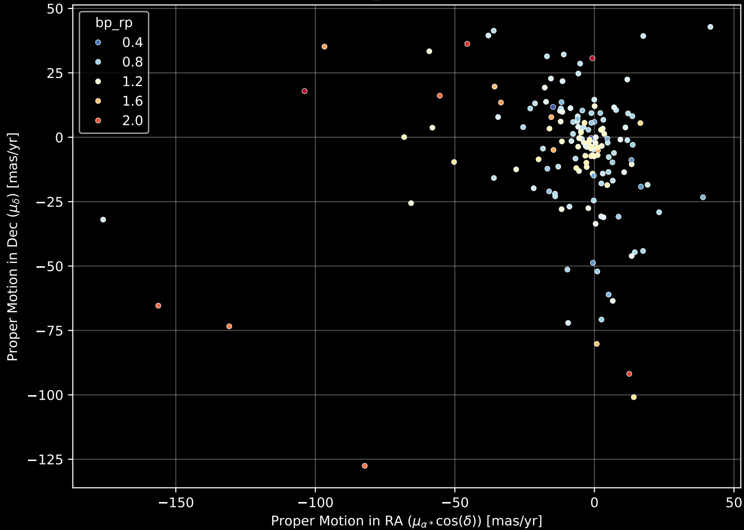
APOGEE DR17 Field: [046+38_MGA] Proper Motion Diagram (n= 157)
