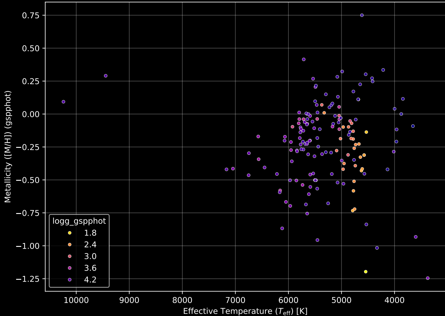
APOGEE DR17 Field: [046+38_MGA] Stellar Population Parameters (n= 157)
